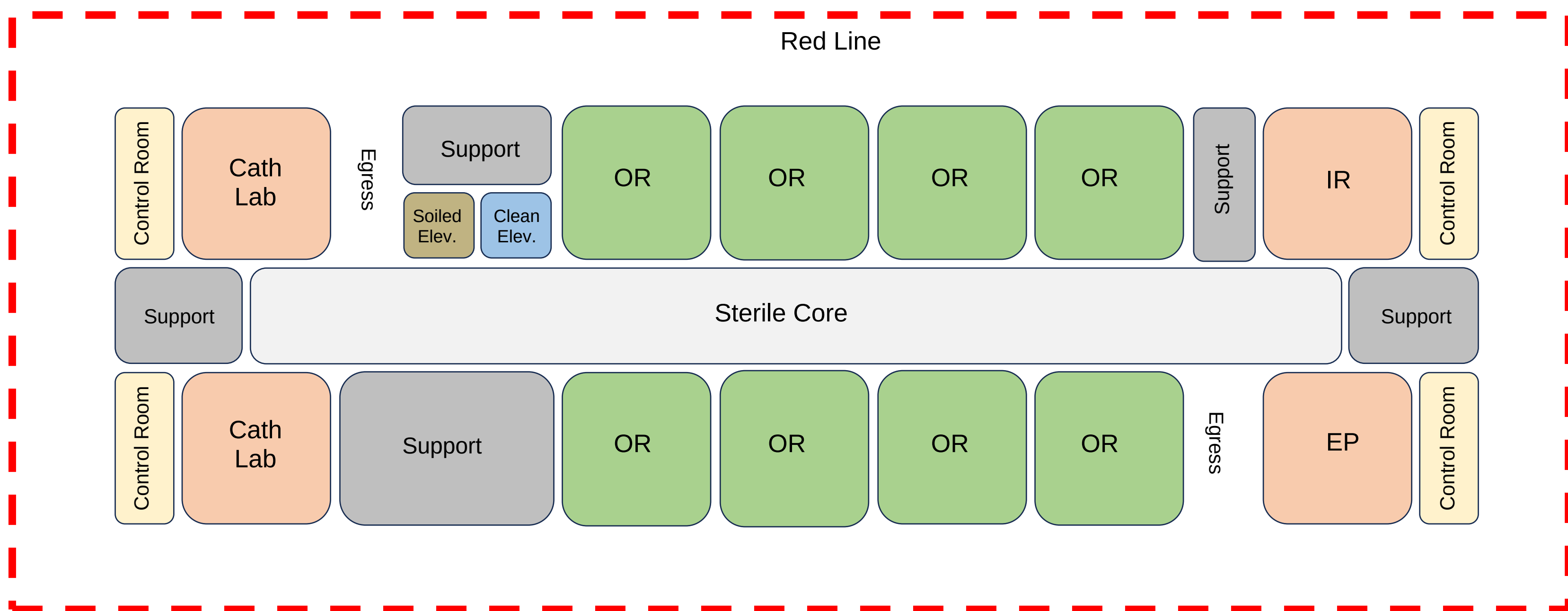
FIGURE 2 - INTEGRATED OPERATING AND INTERVENTIONAL SUITE
